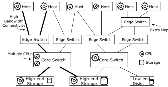
Figure 1. Modern data center with heterogeneous resources
