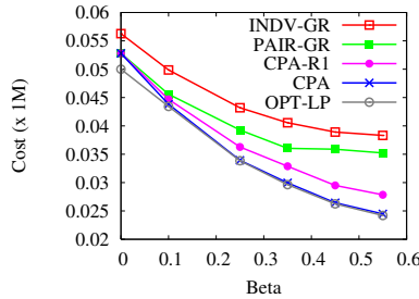
Figure 11. Comparison with OPT-LP
