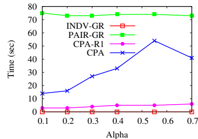
Figure 9. Time with increasing tightness of fit. CPA used 3, 3, 5, 5, 7, 6 rounds.
