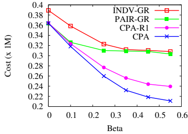
Figure 10. Quality with increasing variance
