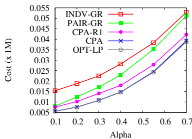
Figure 8. Comparison with OPT-LP
